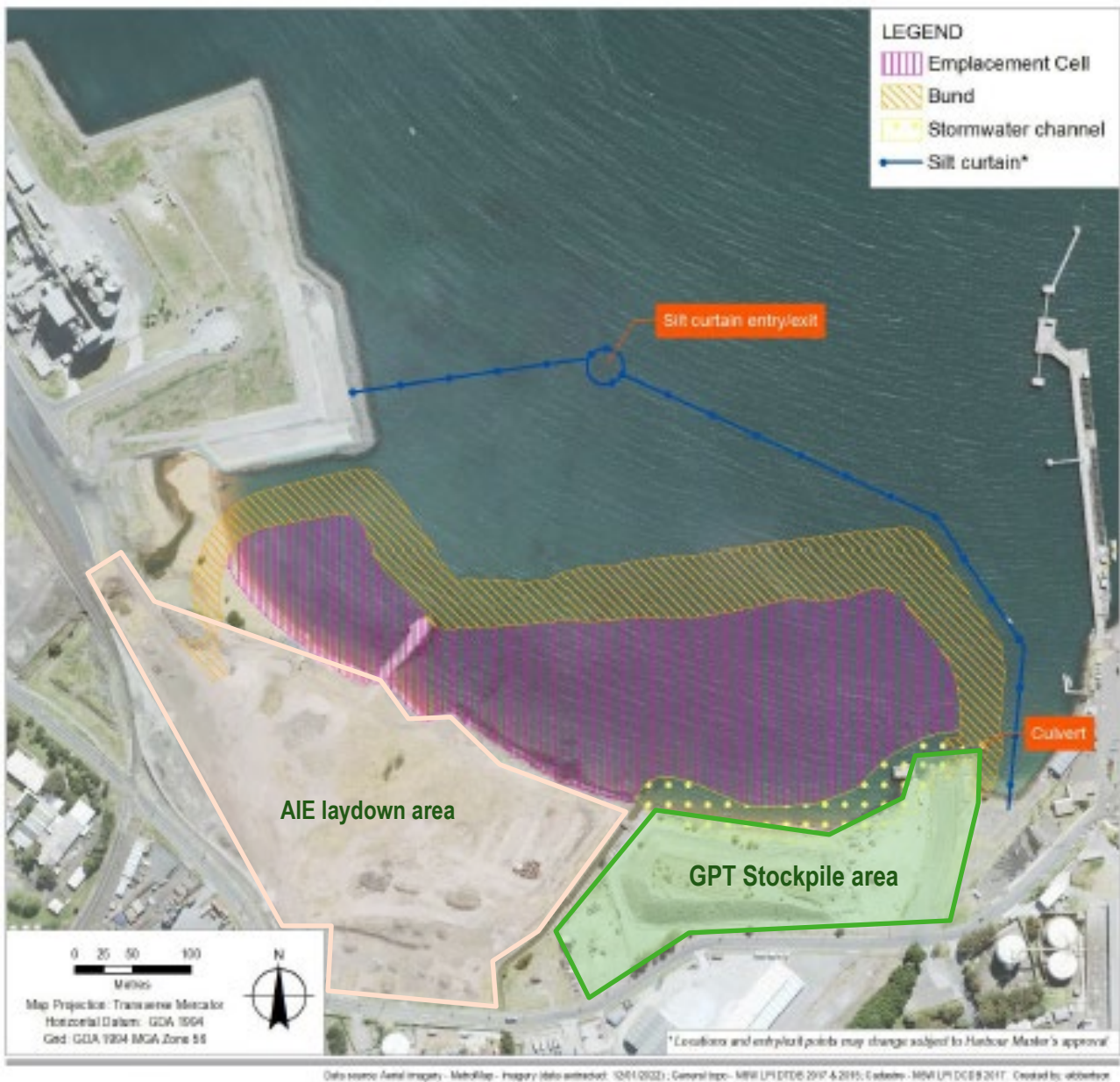
Figure 2. AIE Port Kembla Outer Harbour Emplacement Cell
